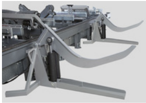
Double-arm hydraulic log loader 1300
